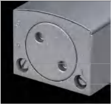
入锁速度调节 latching speed adjusted valve
